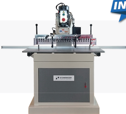
STO-21 23-Spindle Line Bore, Quick-Change
